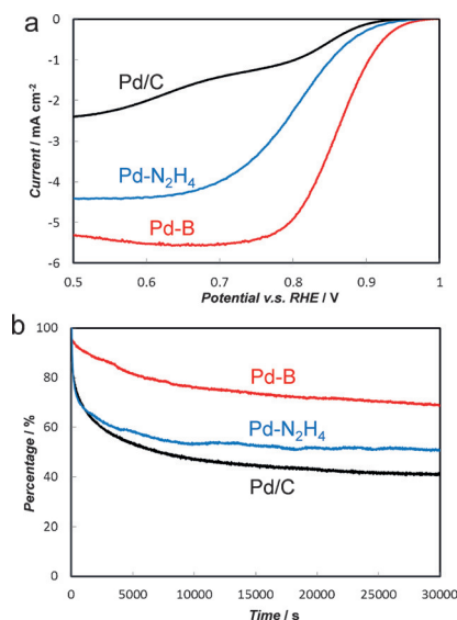
Figure 3. Electrochemical performances of ORR catalysts, Pd–B, Pd–N 2 H 4 , and Pd/C nanoparticles. a) ORR polarization curves were measured in 0.1 M O 2 -saturated KOH solution at a scan rate of 10 mV s −1 . Rotational speed: 1600 rpm. [8,19] b) Chronoamperometry responses were evaluated as percentage of initial current density. The measurements were performed in 0.1 M O 2 -saturated KOH solution at a potential of 0.67 V versus the reversible hydrogen electrode (RHE). Rotational speed: 200 rpm. [8,20]
